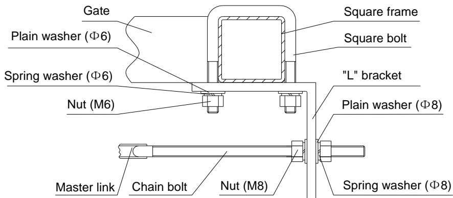
Fig.4 Top view
