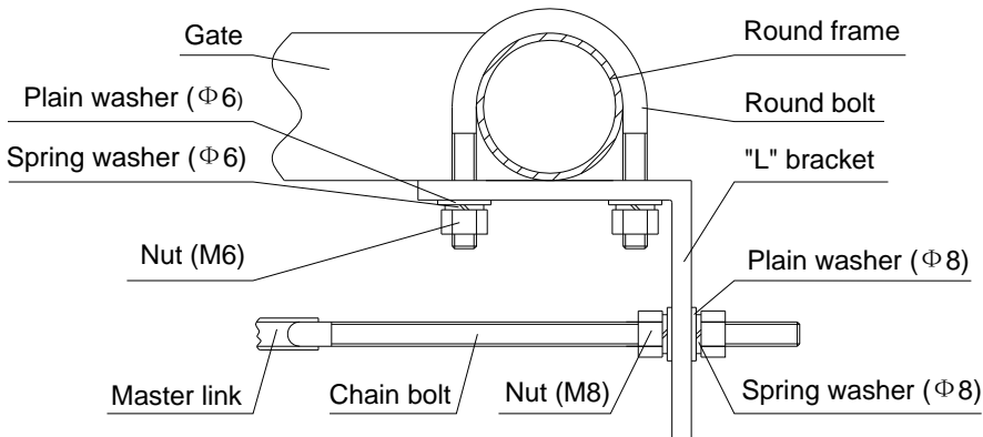
Fig.5 Top view
